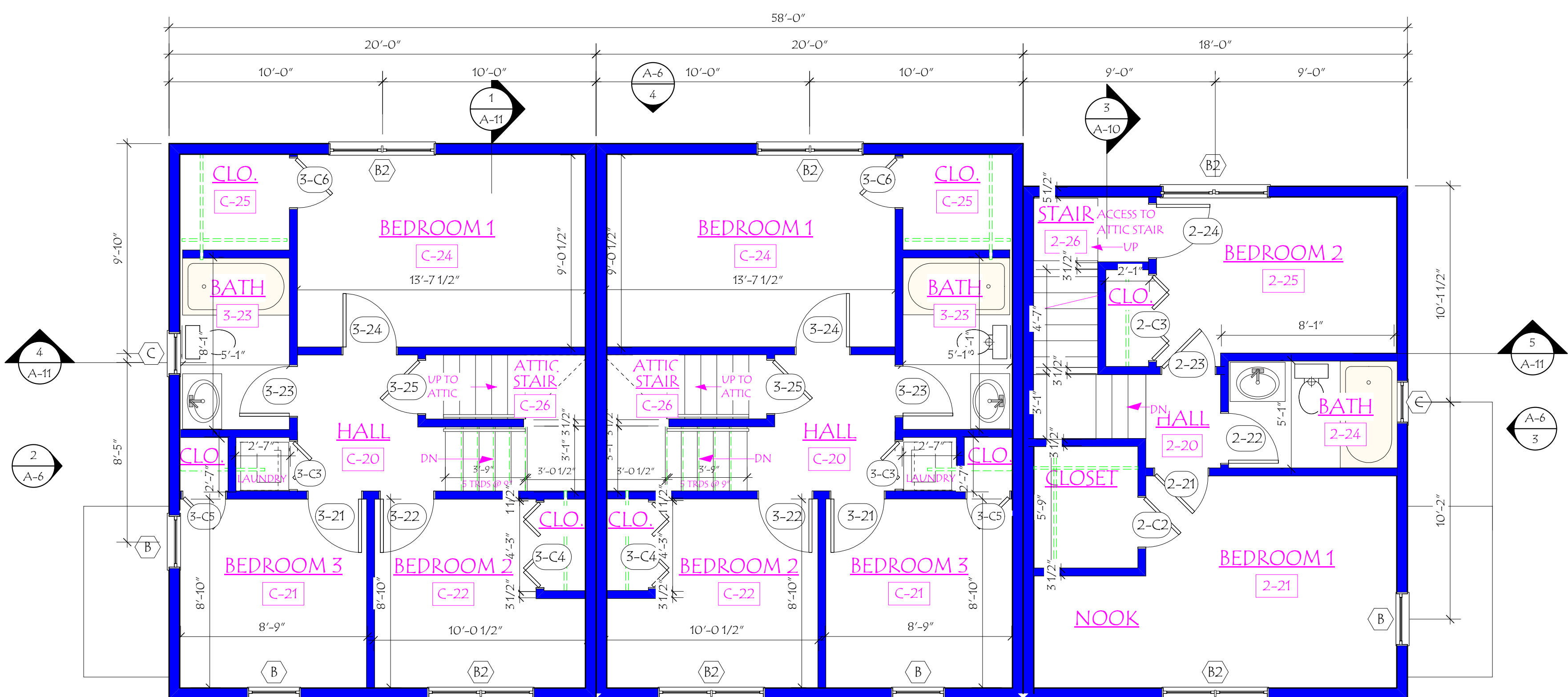
Sm 3BR (3D) Sm 3BR (3E) 2BR (2A) 2 SECOND FLOOR / BUILDING TYPE 3 A-5 Scale: 1/4" = 1'-0"
