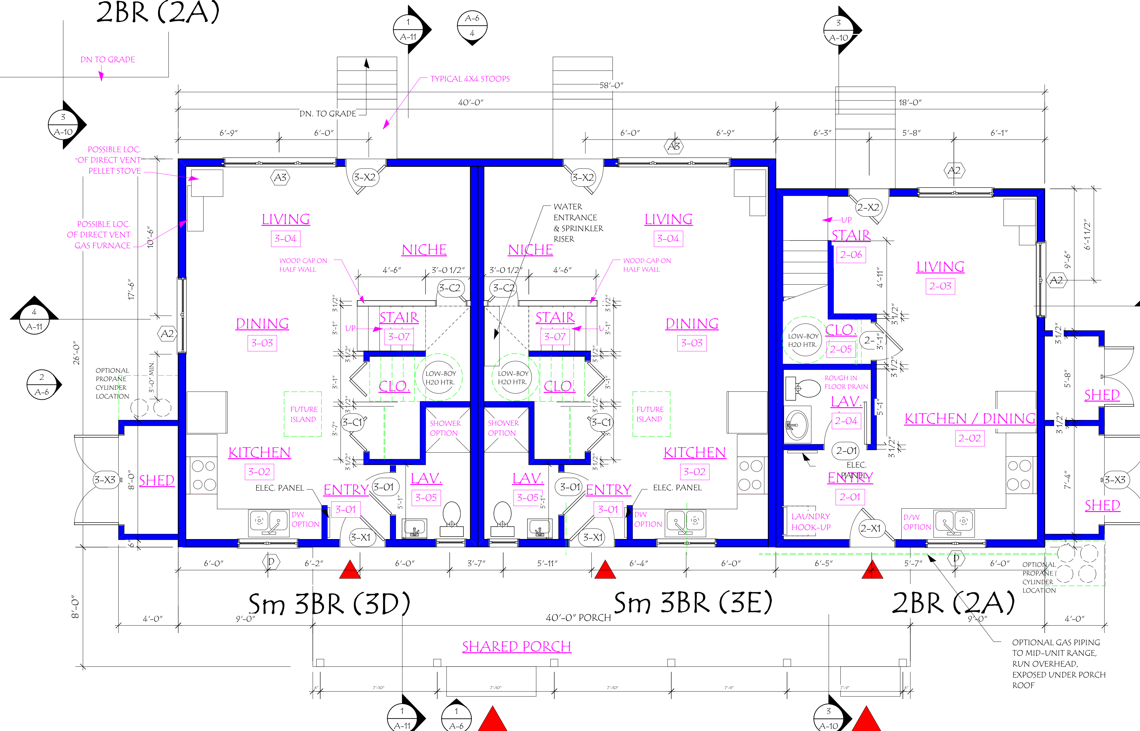
1 FIRST FLOOR / BUILDING TYPE 3 A-5 Scale: 1/4" = 1'-0"
