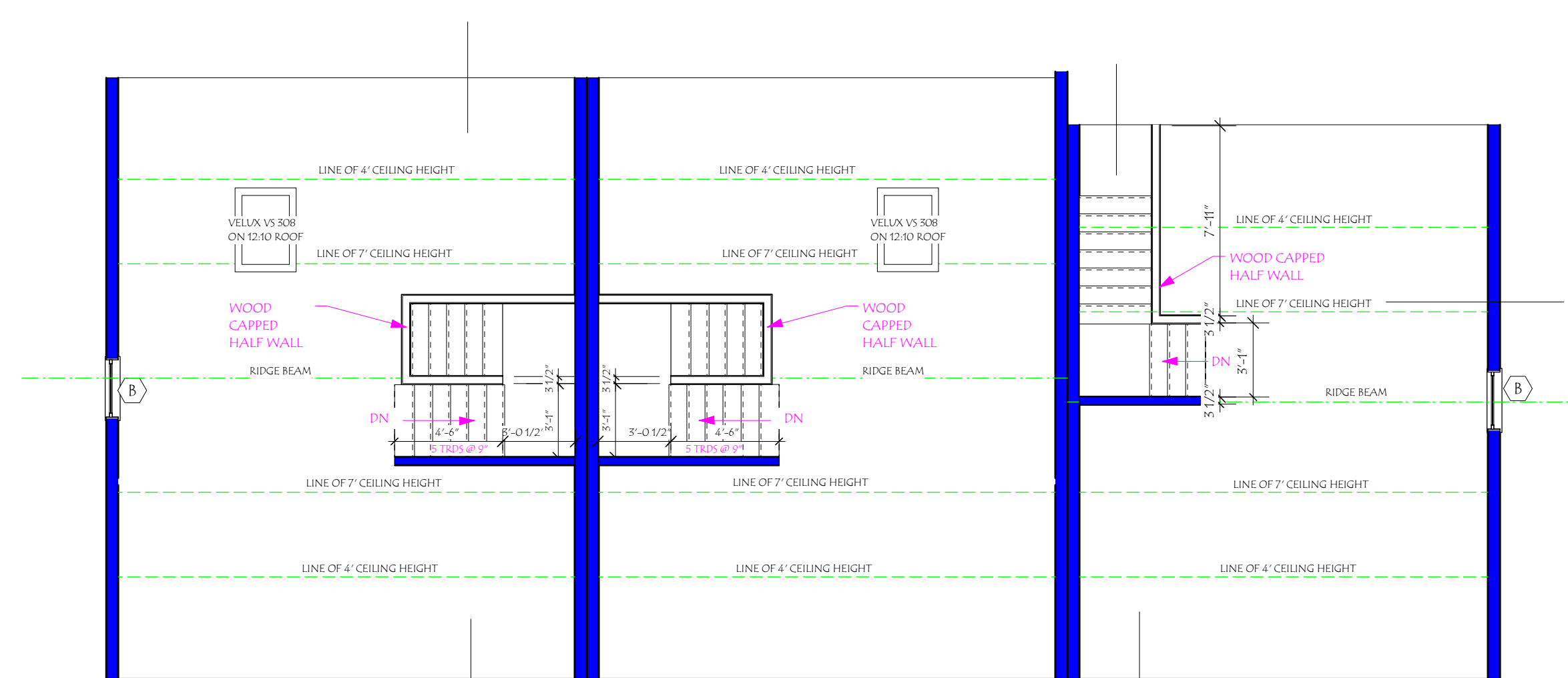
Sm 3BR (3D) Sm 3BR (3E) 2BR (2A) 3 ARCHITECTURAL FINISHES / BUILDING TYPE 3 A-5 Scale: 3/16" = 1'-0"
